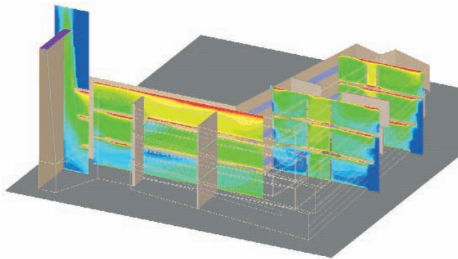
Temperature contours on selected planes in the proposed addition show the range of temperatures that can be expected with natural ventilation
