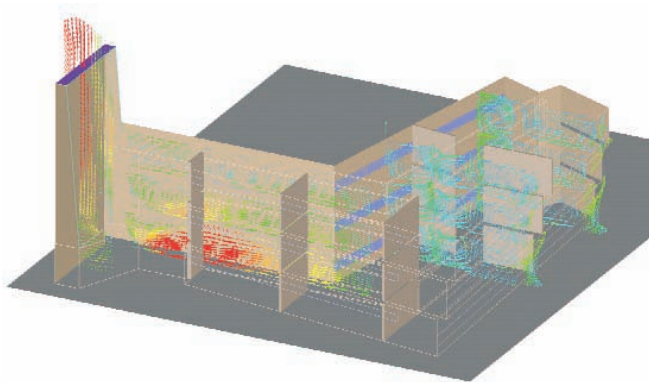
Velocity vectors show the airflow through the building, driven by natural convection
