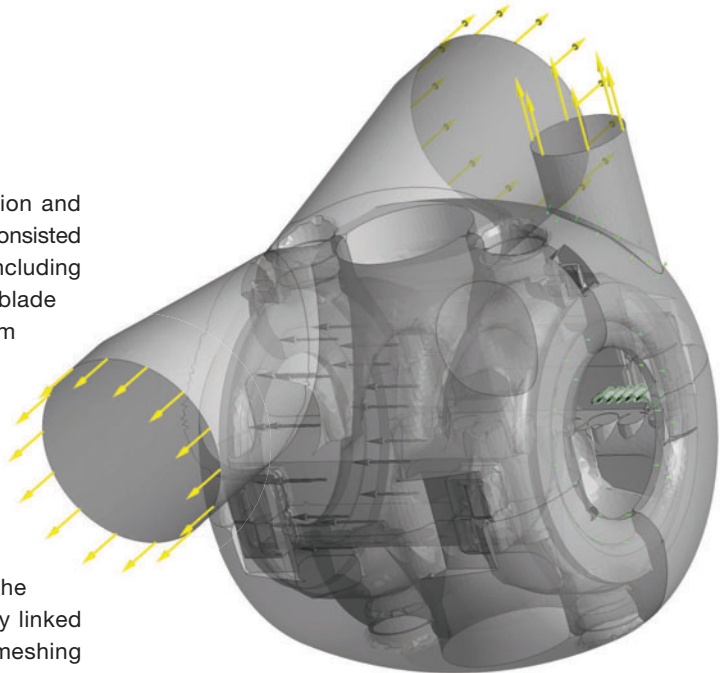
The outlet passage section of the steam turbine
