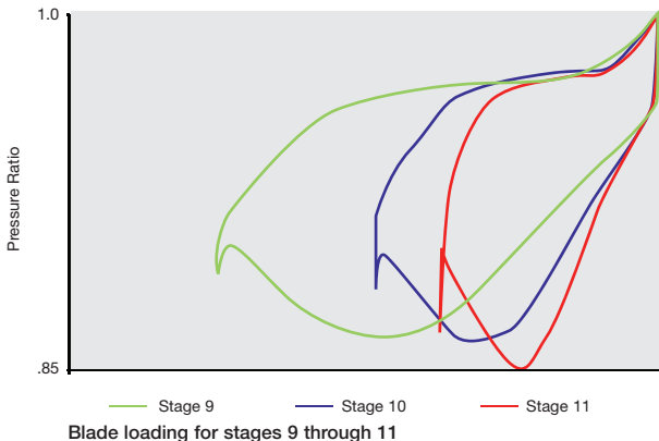
Blade loading for stages 9 through 11
