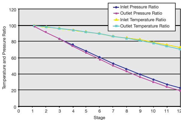
Nondimensional pressure and temperature ratios at the inlet and outlet of each of the 12 stages
