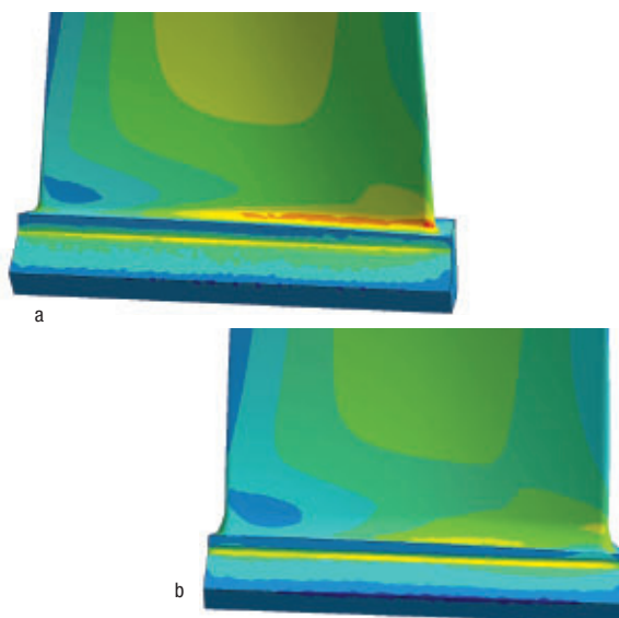
Close-up of the maximum principal stress on the pressure side of (a) the original equipment manufacturer's and (b) the redesigned blades
